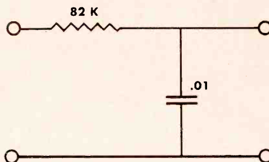
Figure 5. De-attenuation circuit used immediately following the detector of a subcarrier receiver. With the matched pre-attenuation at the transmitter the over-all response is within one db from 50 to 5000 cps.
