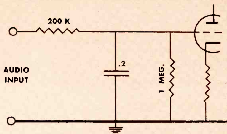
Figure 2. Circuit for producing pre-distortion of audio to convert Phase Modulation to Frequency Modulation.
