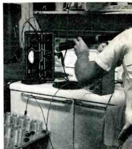
Typical "kitchen" experiment. In this case the "MISSISSIPPI MOOCH" technique is being tried. The distortion meter is first calibrated in the horizontal position, then tipped onto its left side. Distortion measurements are improved due to needle weight by at least 11 RCH.
