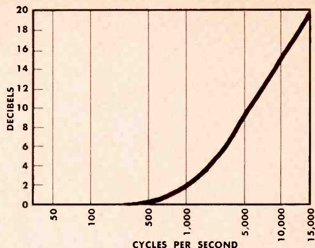
Figure 4. Audio pre-attenuation curve used in the Harkins system of multiplex subcarriers.
